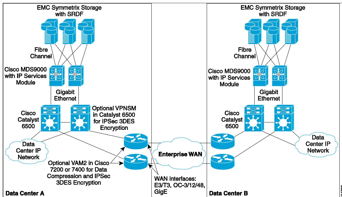
Figure 9: Replication Using FCIP Transport Over WAN Service
