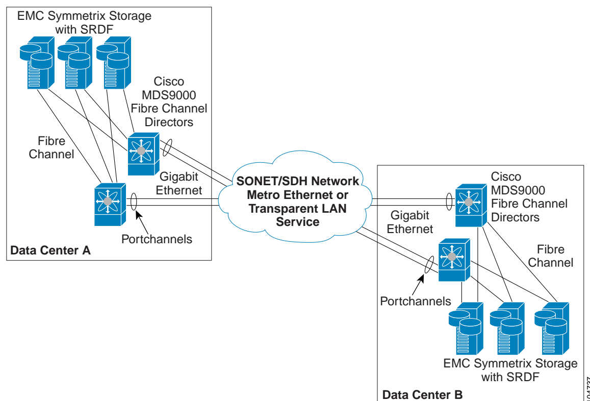
Figure 8: Replication Using FCIP Transport Over SONET/SDH, Metro Ethernet or Transparent LAN Service
