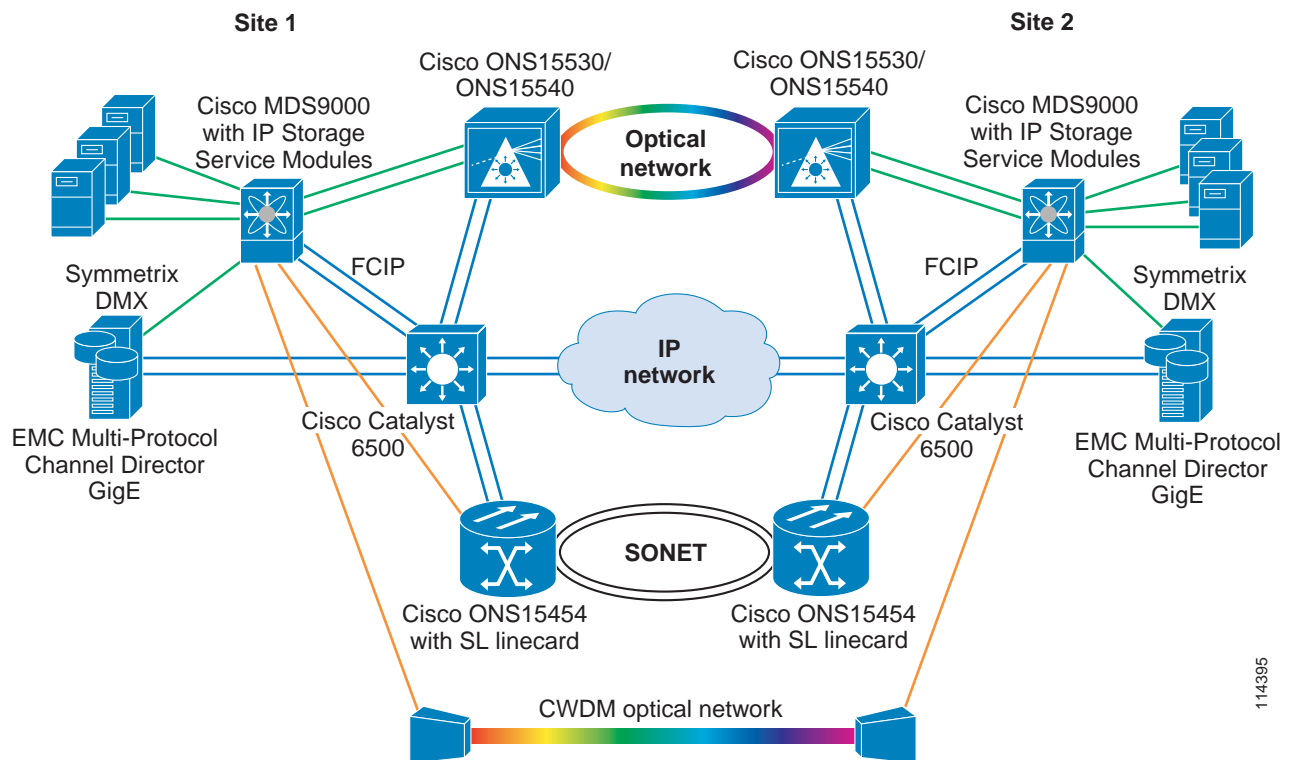
Figure 5: Business Continuance Products from Cisco and EMC
