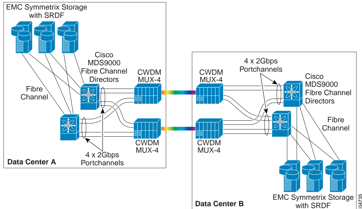
Figure 7: SRDF Synchronous Replication over a Port Channeled MDS 9000 Based Point-to-Point CWDM Network
