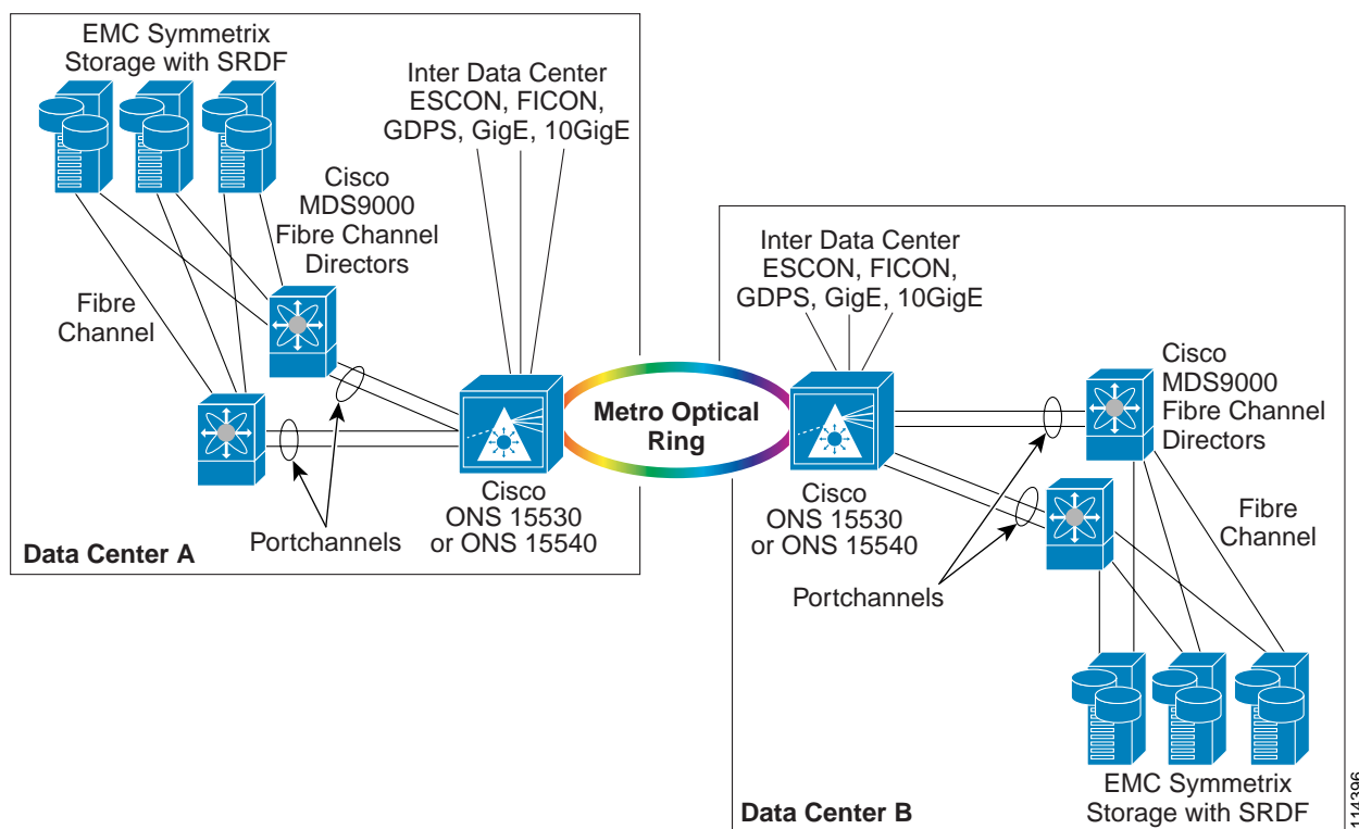
Figure 6: Synchronous Replication over ONS 155x0 DWDM Metro Optical
