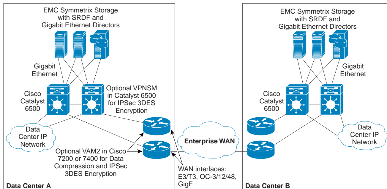
Figure 10: Gigabit Ethernet Director for EMC Symmetrix
